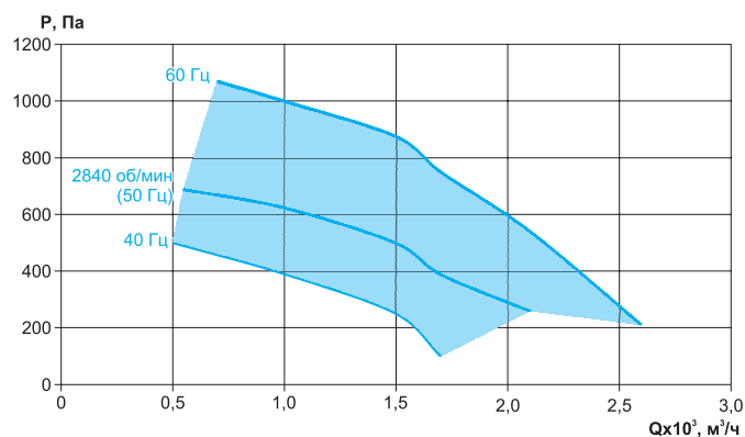
ВРС-К-60-30/25-РЦ-0,75/3000/220-380
